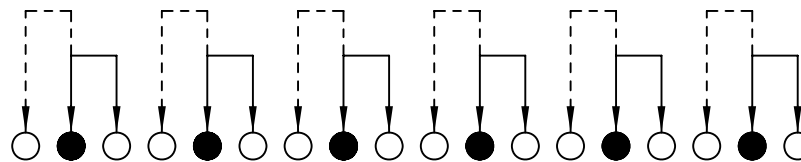
SCHEMATIC (NON-SHORTING)
